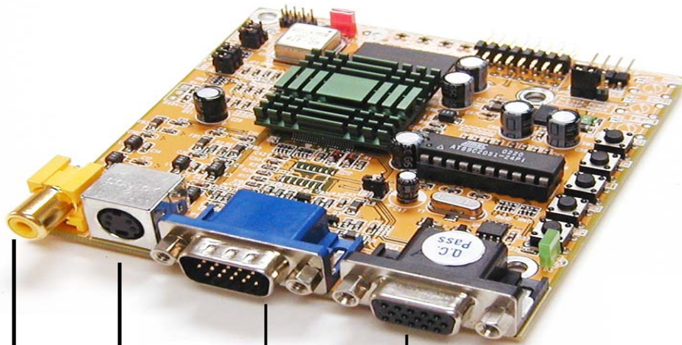
VIDEO OUT S-VIDEO OUT VGA INPUT VGA OUTPUT
